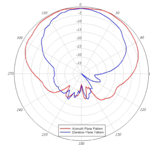
Azimuth and Elevation Radiation Patterns Right Center Antenna - 5 GHz Band
