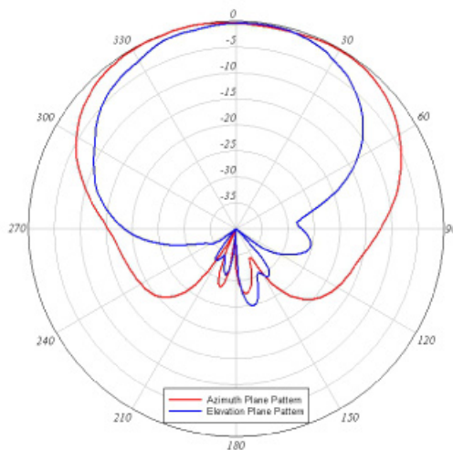
Azimuth and Elevation Radiation Patterns Right Center Antenna - 2.4 GHz Band
