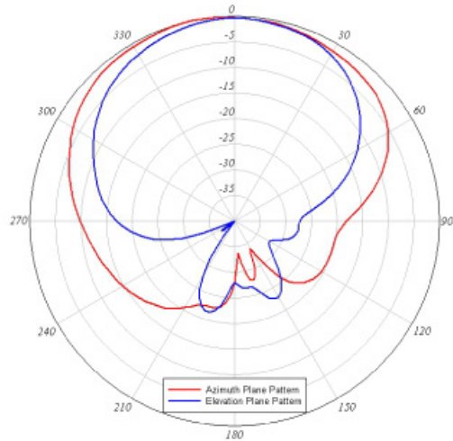
Azimuth and Elevation Radiation Patterns Left Center Antenna - 2.4 GHz Band
