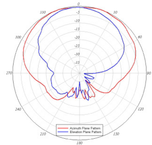
Azimuth and Elevation Radiation Patterns Left Center Antenna - 5 GHz Band
